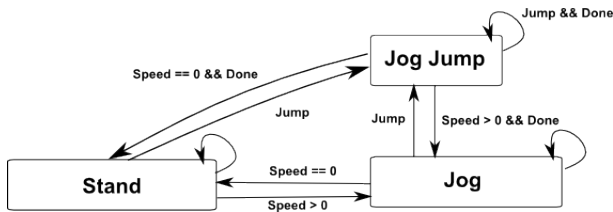
Figure 2: Finite state machine used for the NoMotion, Switch, Blend, and Cape conditions. Note that standing and jogging automatically loop where jumping only repeats based on boolean state variables.
